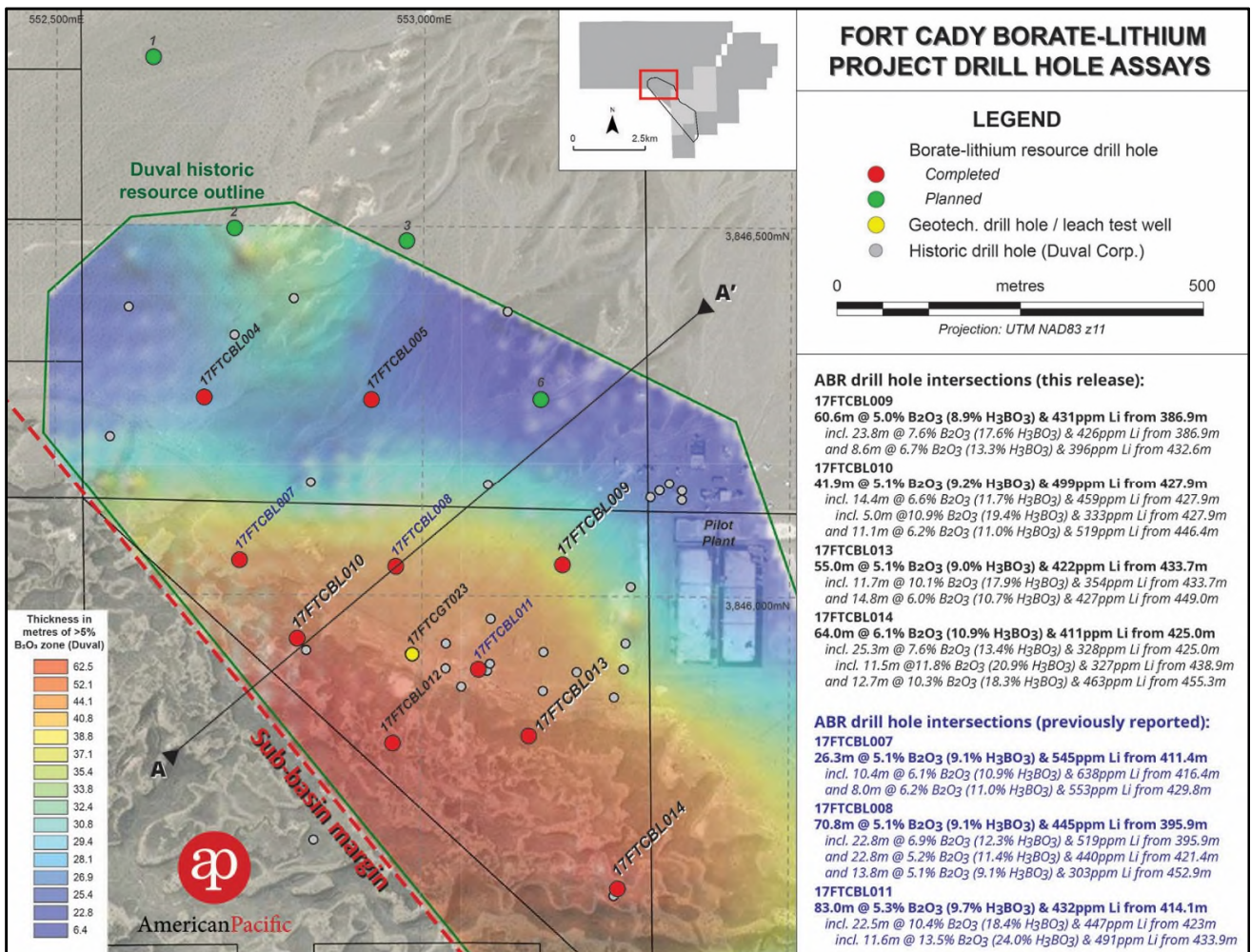
Figure 1. Drill hole locality map highlighting location of drill holes 17FTCBL009, 17FTCBL010, 17FTCBL013 and 17FTCBL014. Location of cross-section (figure 2) highlighted (A – A').
