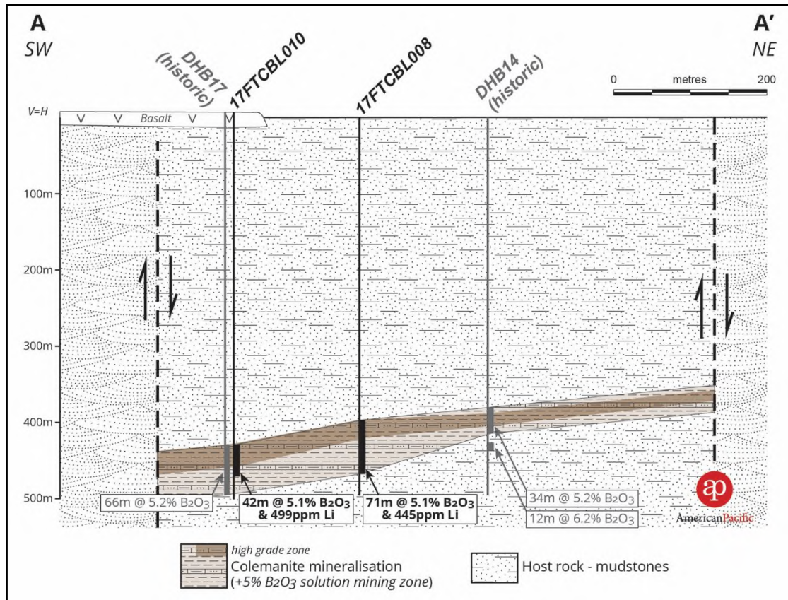
Figure 2. Schematic cross-section through the Fort Cady colemanite ore body (view looking northwest).
