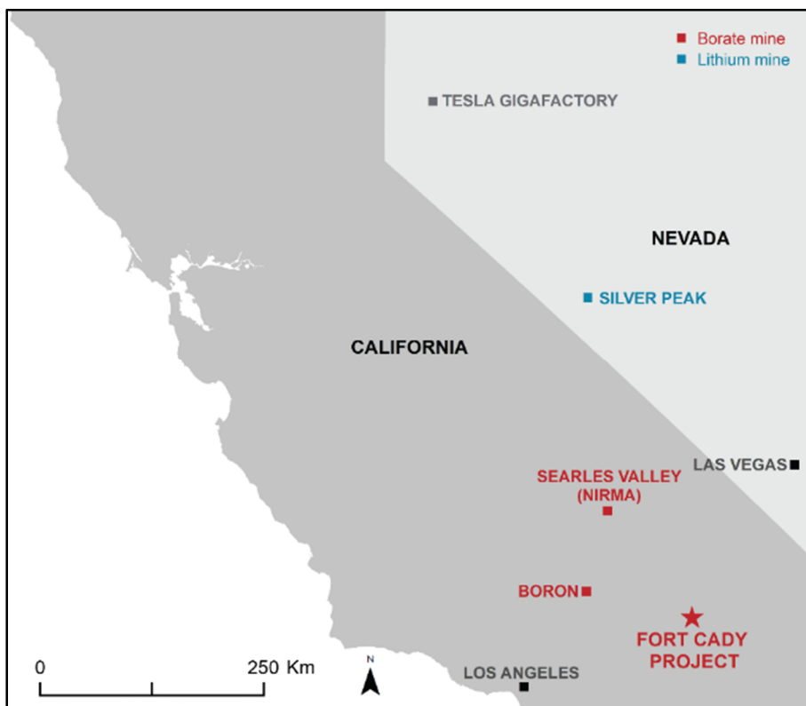
Figure 3. Location of the Fort Cady Borate and Lithium Project, California USA.
